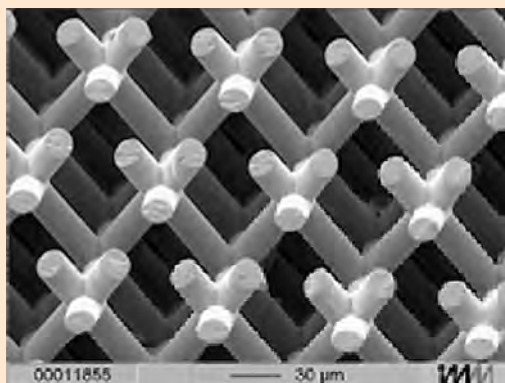
Figure 5. The “three-cylinder” photonic crystal made from negative tone resist [1].
