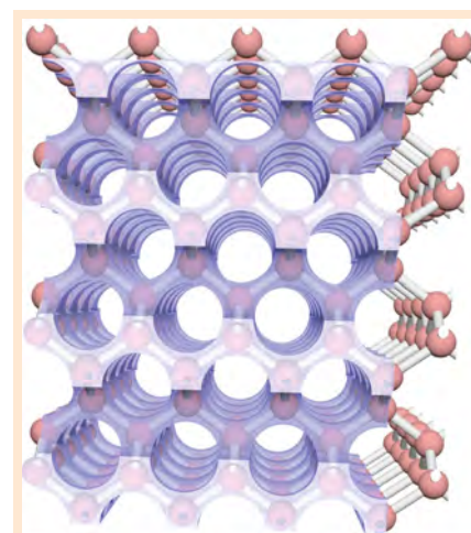
Figure 1. A “ball and the stick” model of the diamond structure, viewed from an angle such that the channels along a [110] direction are observable. Shrinking the size of the “balls”, while keeping the “sticks” and “3-cylinder” diamond structure with “air-cylinder”.
