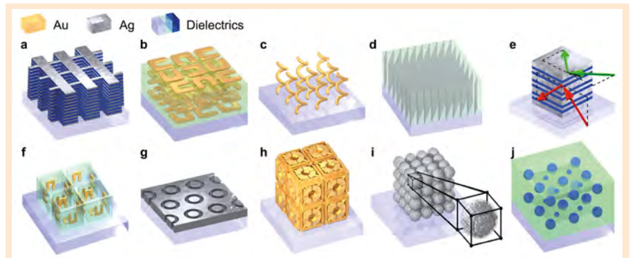
Figure 8. 3D Photonic-Metamaterials Structures. This figure is taken from the article in Nature Photonics 5, 523 (2011) written by Soukoulis and Wegener [4].
