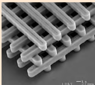
Figure 4. Electron-microscope image of a “woodpile” photonic crystal made by silicon with a complete band gap at 12 μm [1].
