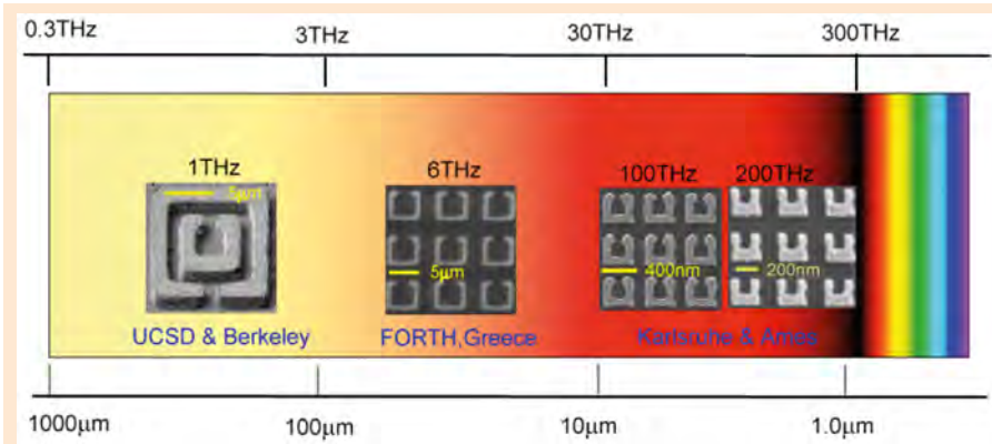
Figure 6. The operation frequency of magnetic metamaterials increased rapidly. The structures operating at 1, 6 and 100 THz frequency, respectively, were fabricated in 2004, and the one at 200 THz in 2005.
